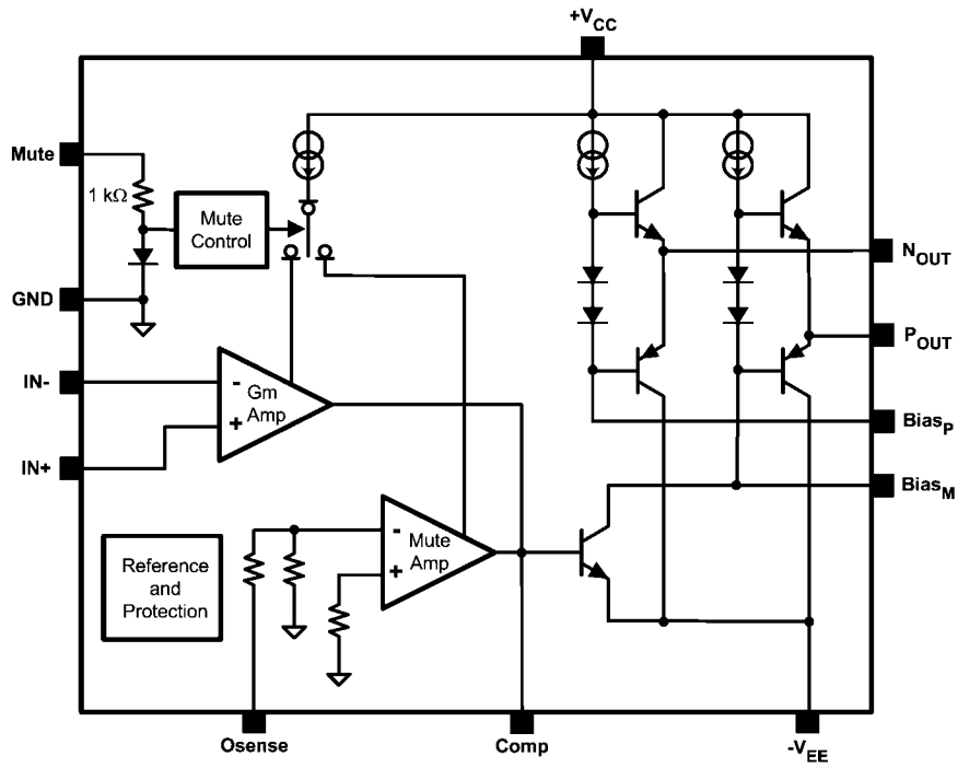
FIGURE 2. LME49830 Simplified Block Diagram
