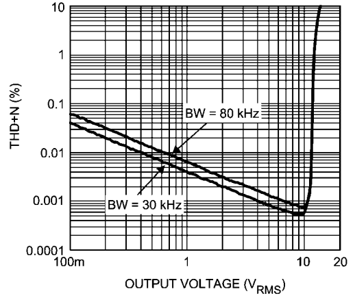
THD+N vs Output Voltage +V_{CC} = -V_{EE} = 20V, f = 1kHz
