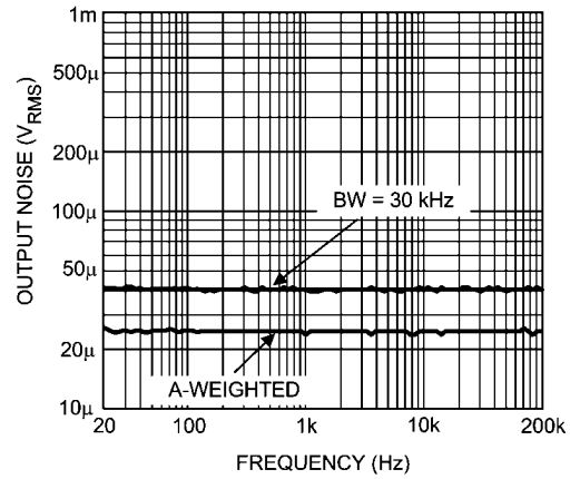
Noise Floor +V_{CC} = -V_{EE} = 100V, V_{IN} = 0V
