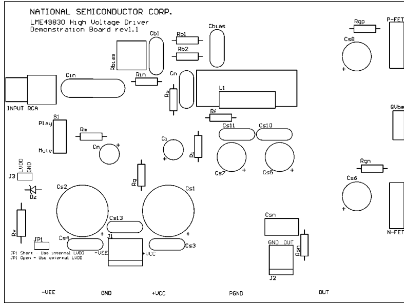
Top Silkscreen
