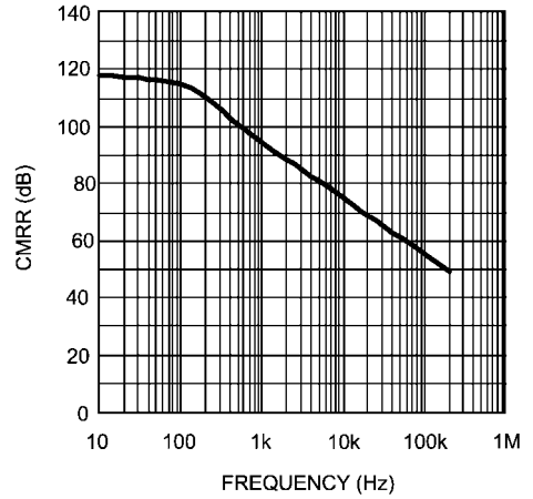
CMRR vs Frequency +V_{CC} = -V_{EE} = 100V
