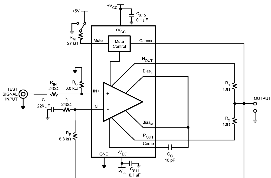
FIGURE 3. LME49830 Test Circuit Diagram
