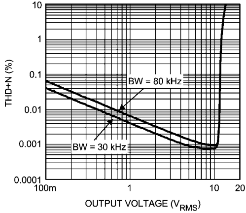
THD+N vs Output Voltage +V_{CC} = -V_{EE} = 20V, f = 20Hz
